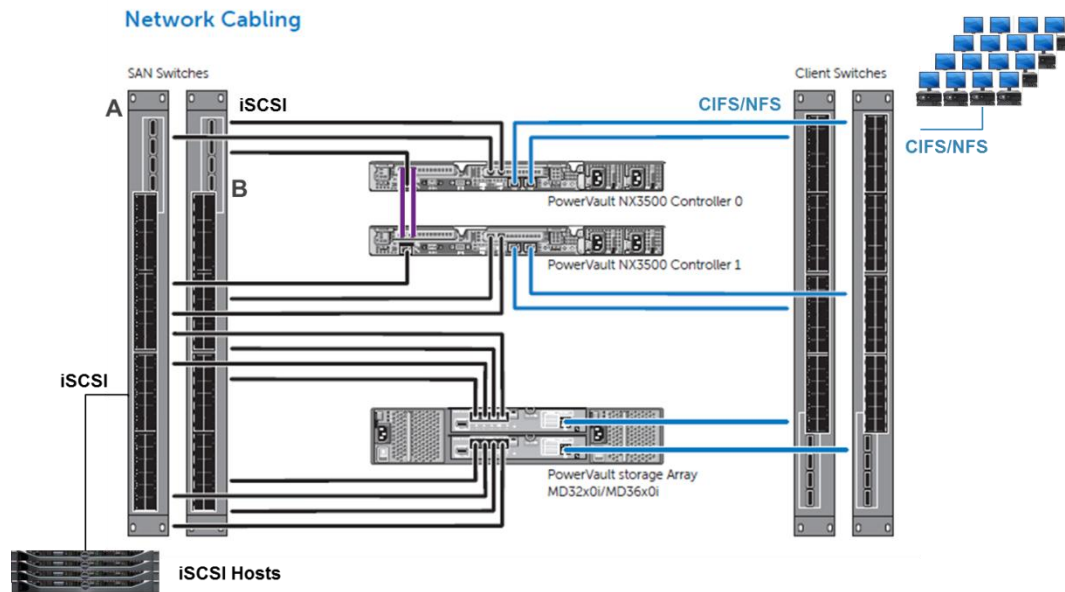
PowerVault NX3500 Network Cabling
