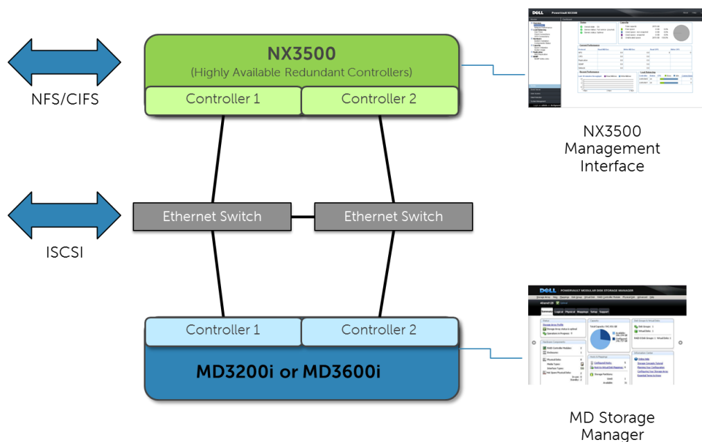
PowerVault Unified Storage Solution - High Level Logical Diagram
